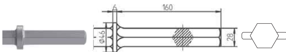
Hexagonal 28 mm + collar (ref.321H, 351H, 373H)
